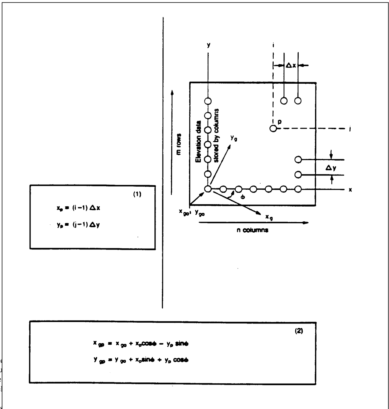
Figure 5.--Geometry and nomenclature of the 7.5-minute Digital Elevation Model file.
